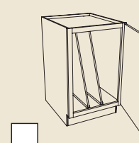
Tray Base Block 3030 Works well for organizing canvases and frames.
