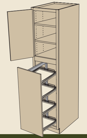
4. Utility Pull-out Pantry with Soft-close Block 5185
