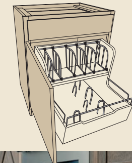
2. Base Plastic Ware Storage Block 4067
